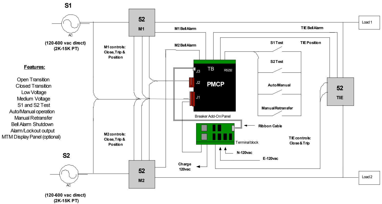
PMCP and Breaker Add-On Panel operating a Main-Tie-Main
